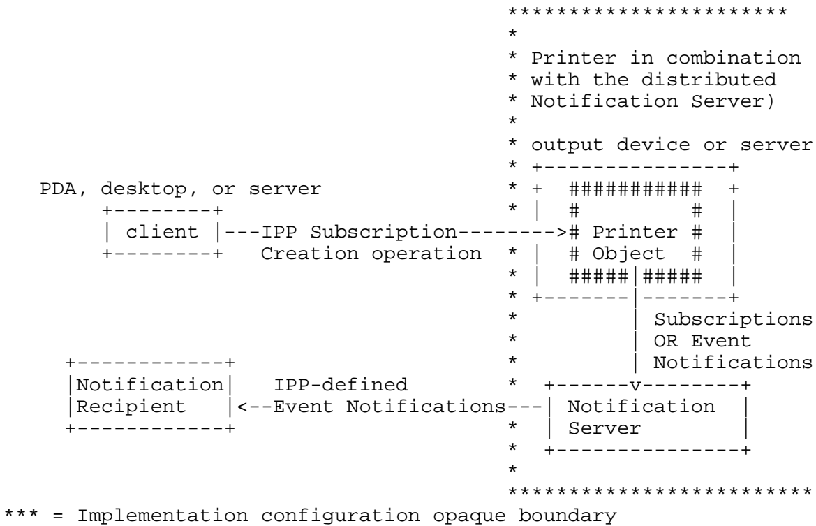
Figure 3 – Opaque Use of a Notification Server Transparent to the Client
