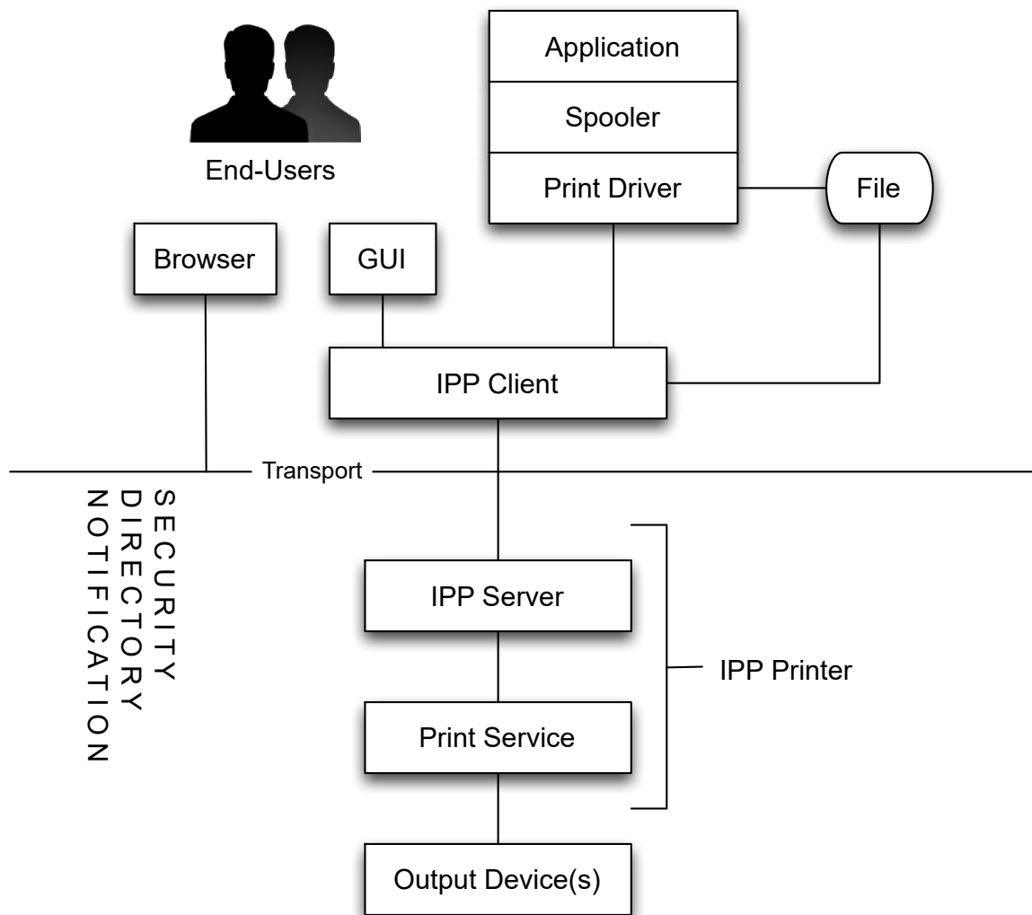
Figure 1 - IPP General Model [STD92]
