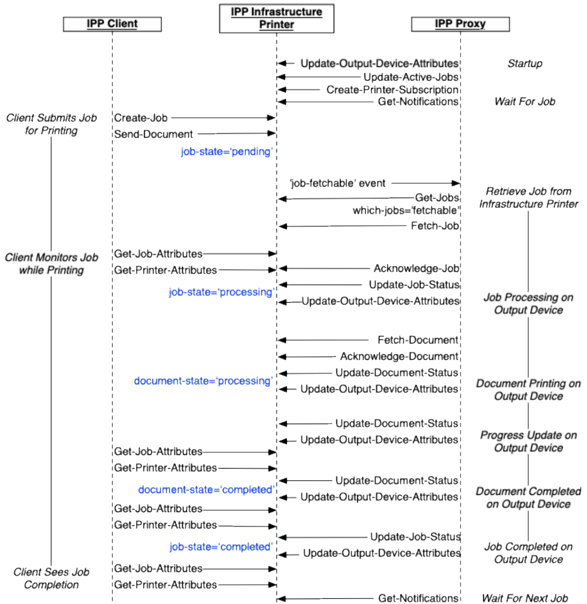
Figure 4 - Non-Release Job Processing Sequence Diagram
