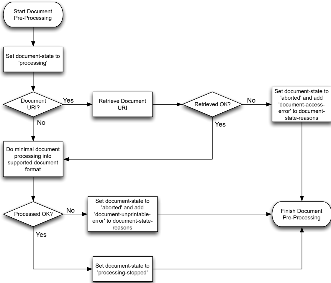
Figure 7 - Infrastructure Printer Document Pre-Processing Flowchart
