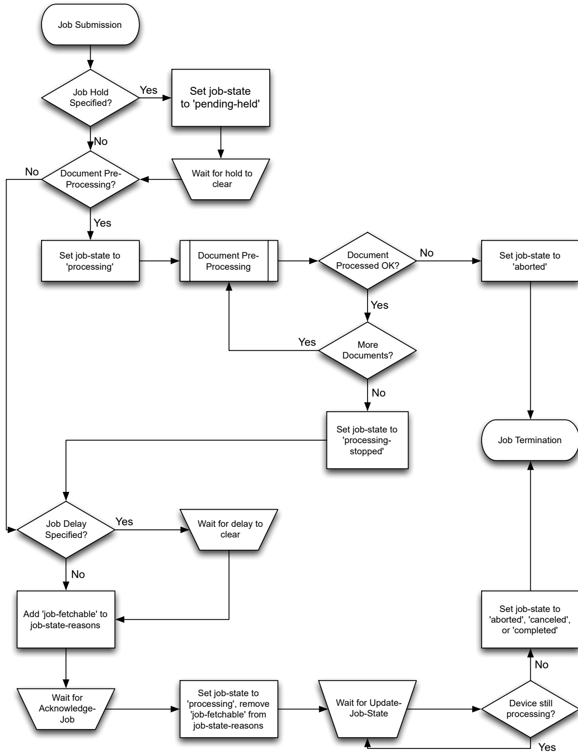
Figure 6 - IPP Infrastructure Printer Job Processing Flowchart
