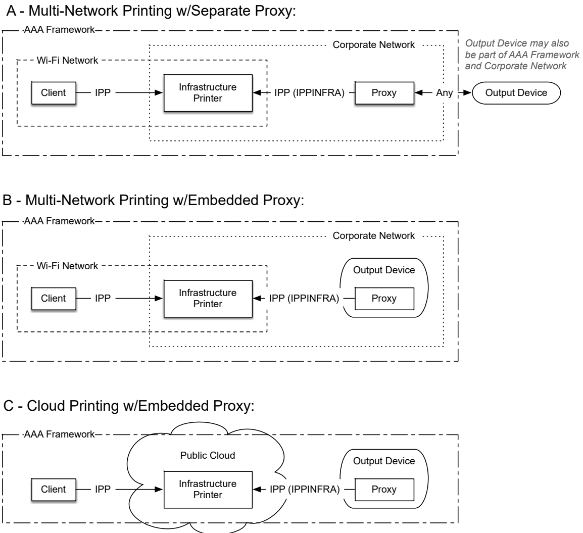
Figure 2 - Shared Infrastructure IPP Model
